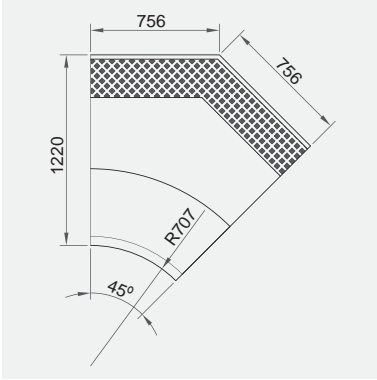
GARDENYA 112 - 45° İç Köşe GARDENIA 112 - 45° Internal Corner
