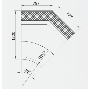
GARDENYA 122 - 45° İç Köşe GARDENIA 122 - 45° Internal Corner
